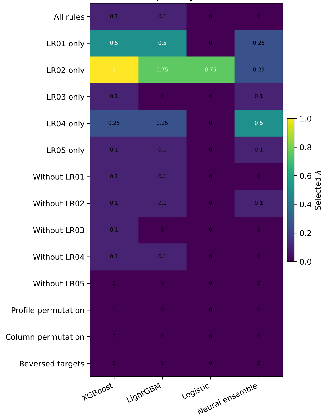
(a) Selected penalty
