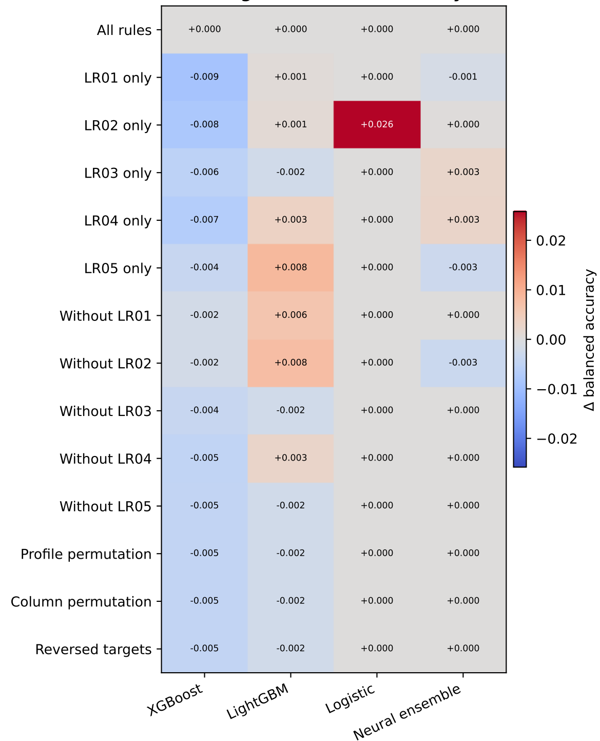
(b) Change in balanced accuracy vs all rules
