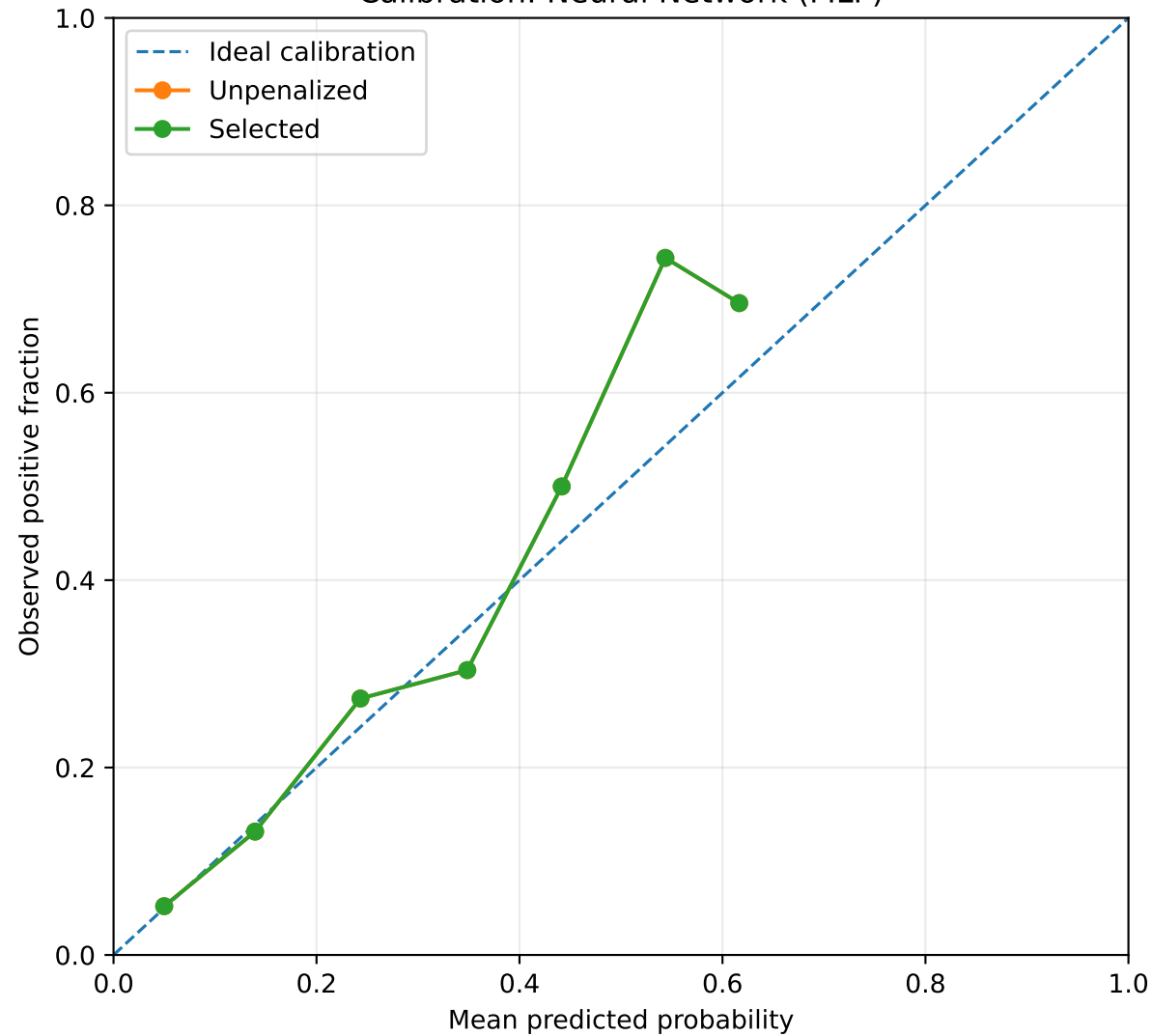
Calibration: Neural Network (MLP)
