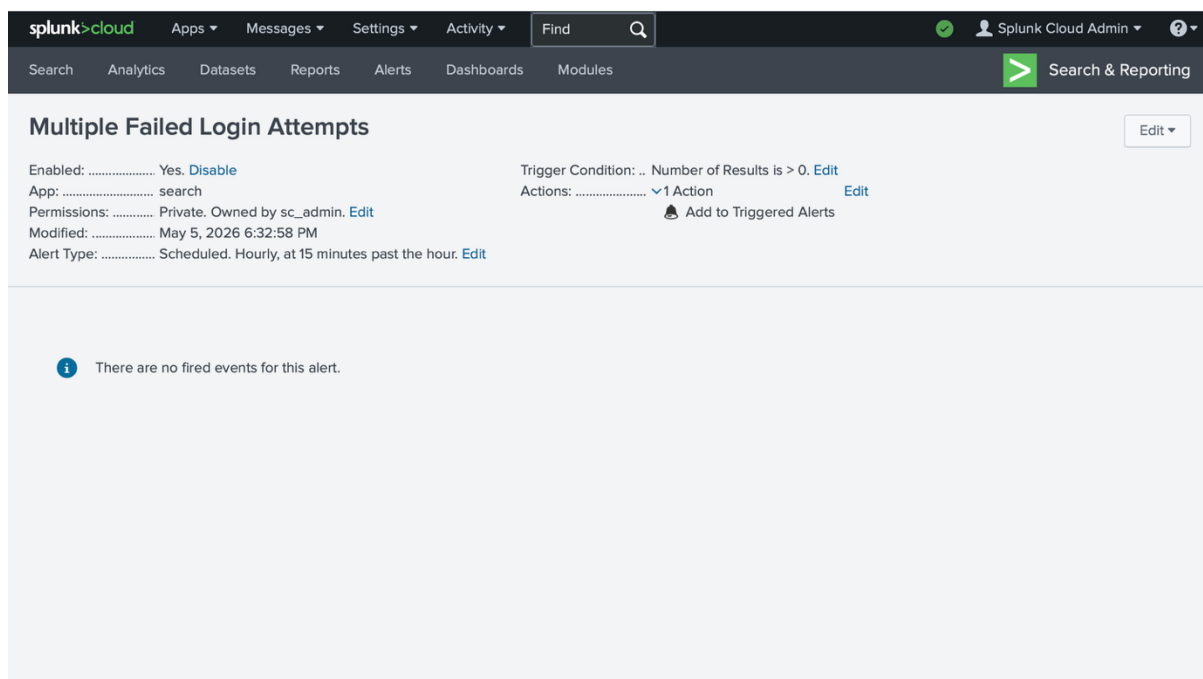
Figure 3: Scheduled alert configured for detecting multiple failed login attempts.
