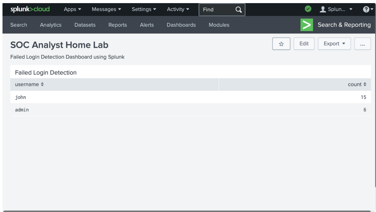
Figure 2: Failed Login Detection Dashboard created in Splunk Cloud.
