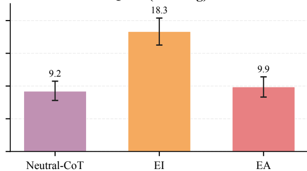
Qwen (thinking)
