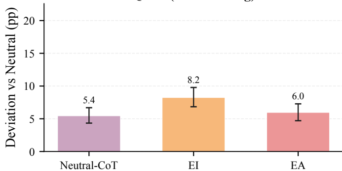
Qwen (non-thinking)
