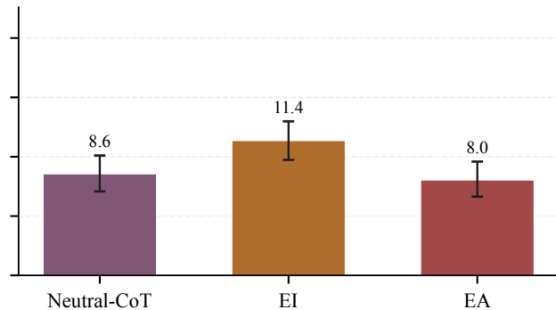
o4-mini
