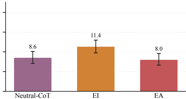
o4-mini
