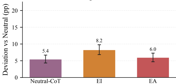
Qwen-N
