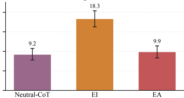
Qwen-T
