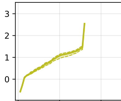
Mistral-7B-Instruct-v0.2
