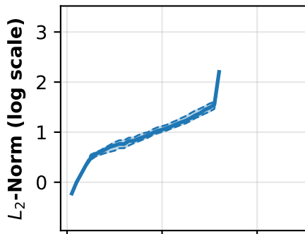
Qwen2.5-14B-Instruct
