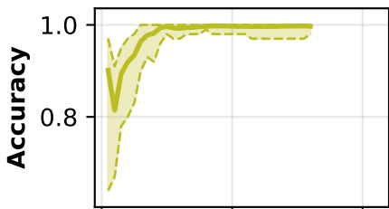
Mistral-RB
