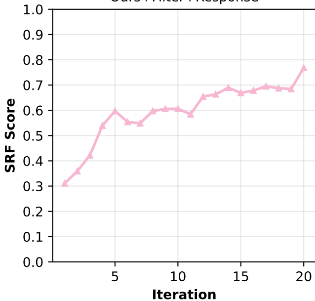
Ours+Filter+Response
