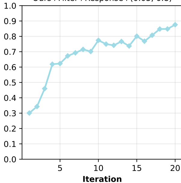
Ours+Filter+Response+(0.05, 0.8)
