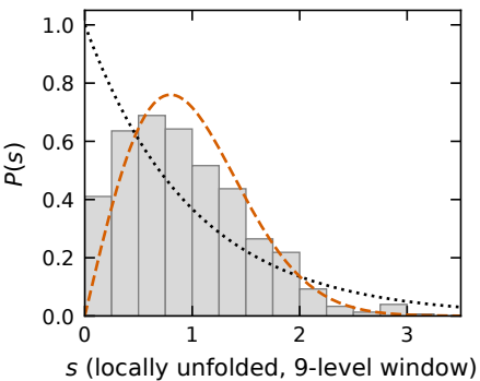
\langle s^2 \rangle = 1.72 (Poisson 2, GOE 1.27)
