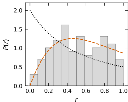
N = 10^4 outside the bracket, 119 r \langle r \rangle = 0.519 \pm 0.024
