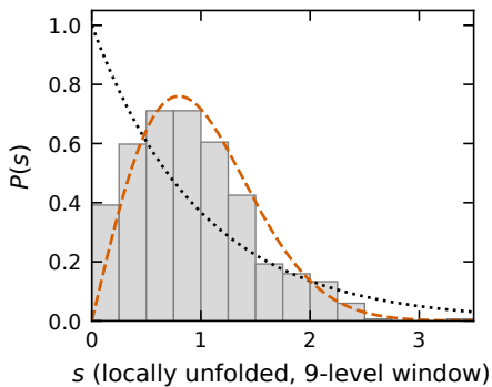
\langle s^2 \rangle = 1.76 (Poisson 2, GOE 1.27)
