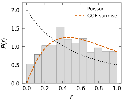
N = 10^3 elliptical, 611 levels \langle r \rangle = 0.508 \pm 0.010
