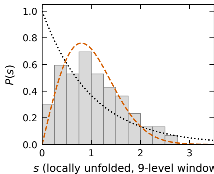
\langle s^2 \rangle = 1.48 (Poisson 2, GOE 1.27)
