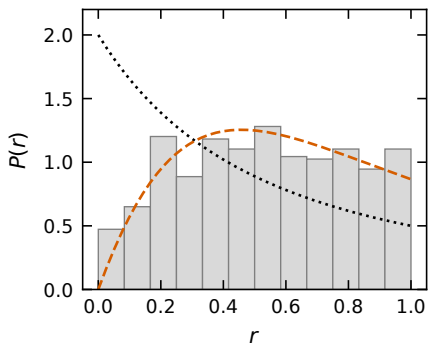
N = 10^3 circular, 611 levels \langle r \rangle = 0.533 \pm 0.011
