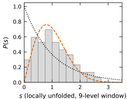
\langle s^2 \rangle = 1.48 (Poisson 2, GOE 1.27)
