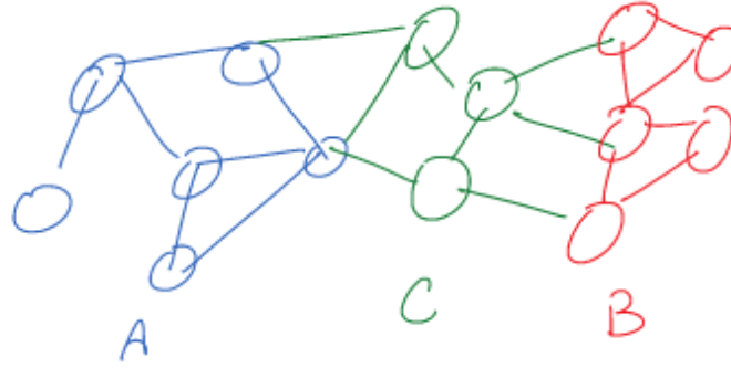
Figure 9.2: MRF Theorem
