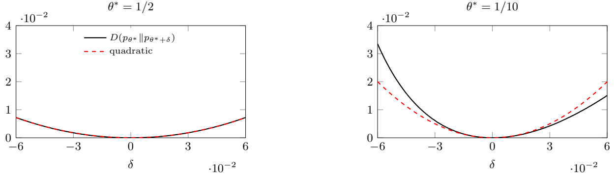
Figure 1.5: Relative entropy between two coins whose biases differ by \delta , in nats, with the quadratic approximation (1.23) dashed. Both panels use the same scales. The valley is steeper around \theta^* = 1/10 than around \theta^* = 1/2 , so the same change in bias is easier to detect in a lopsided coin, and its Fisher information is larger. The left panel is symmetric in \delta and the right one is not, a reminder that (1.23) describes only the immediate neighborhood of \theta^* .
