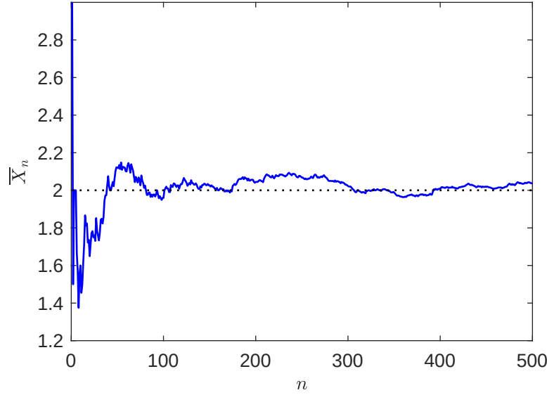
Figure 4: \bar{X}_n based on X_i \sim \text{Poi}(2) as a function of n .
