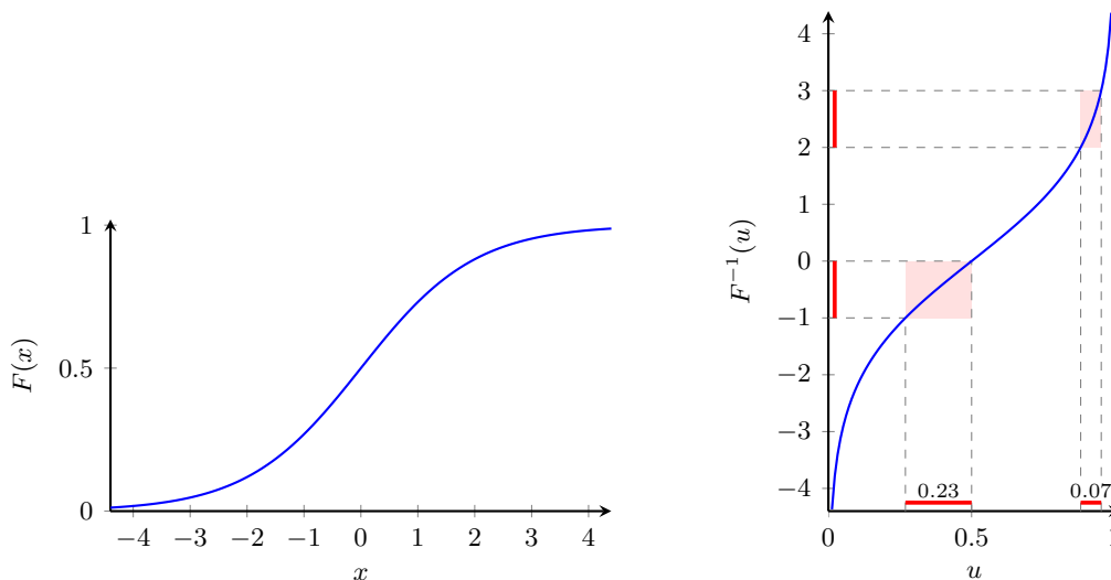
Figure 1: A CDF (left) and its inverse (right), drawn to the same scales: the u axis carries the same scale as the F axis, and the F^{-1} axis the same as the x axis. Two intervals of equal width are shaded on the F^{-1} axis. The values of u mapped into them, marked on the u axis, occupy lengths 0.23 and 0.07, which are the probabilities that X falls in the two intervals.
