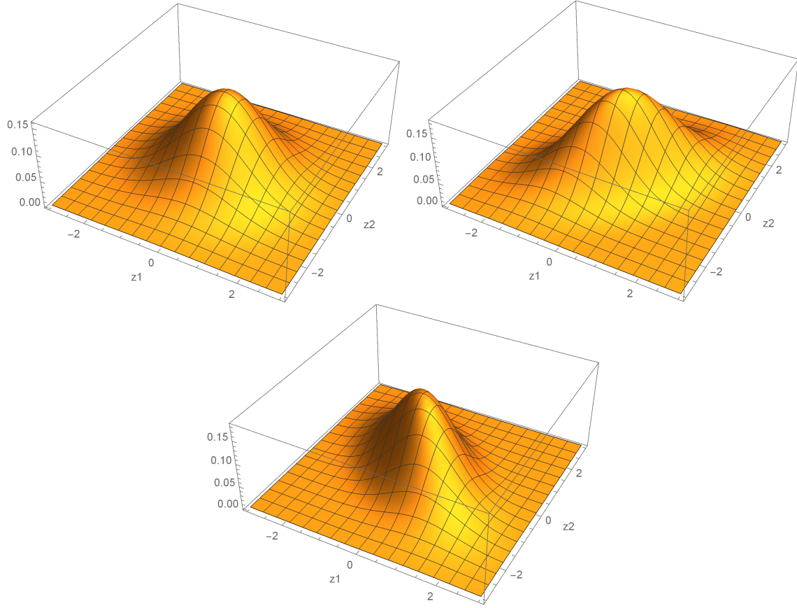
Figure 3: Bivariate Normal pdfs with \mu_X = \mu_Y = 0 , \sigma_X = \sigma_Y = 1 , with \rho = 0 (uncorrelated), \rho = .5 (positively correlated), and \rho = -.5 (negatively correlated), respectively.
