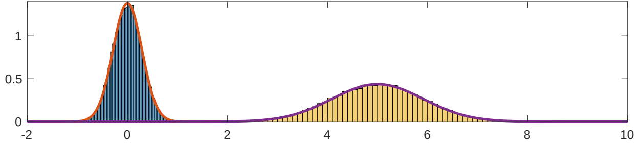
Figure 5: The normalized histograms for \sqrt{n}(\bar{X}_n - \mu) and the pdf of \mathcal{N}(0, \sigma^2) (on the left) and the normalized histogram for S_n and the pdf of \mathcal{N}(n\mu, n\sigma^2) (on the right) for uniform X_i with \mu = 1/2 and \sigma^2 = 1/12 and with n = 10 .
