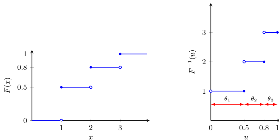
Figure 2: The CDF of \text{Cat}(0.5, 0.3, 0.2) (left) and its inverse (right), drawn to the same scales. The jump of height \theta_i that the CDF makes at i becomes the step of width \theta_i on which F^{-1} equals i , so a uniform U produces i with probability \theta_i . At a jump, F^{-1} takes the lower of the two values, since it is the first value at which the CDF reaches u .
