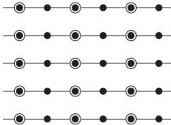
YUV4:2:2 采样
