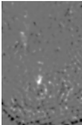
Delta response (L1, sharpened)
