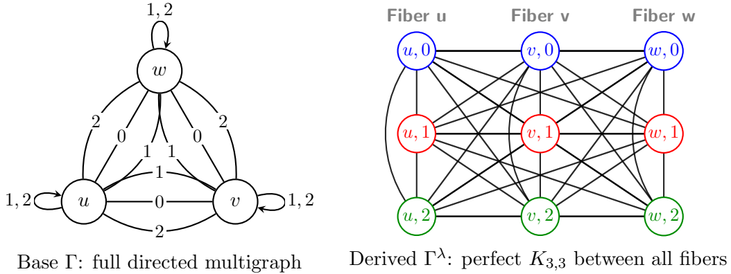
Figure 4.6: Voltage graph and derived cover for the loopfree, undirected quantum graph on M_3(\mathbb{C}) with m = 8 quantum edges.
