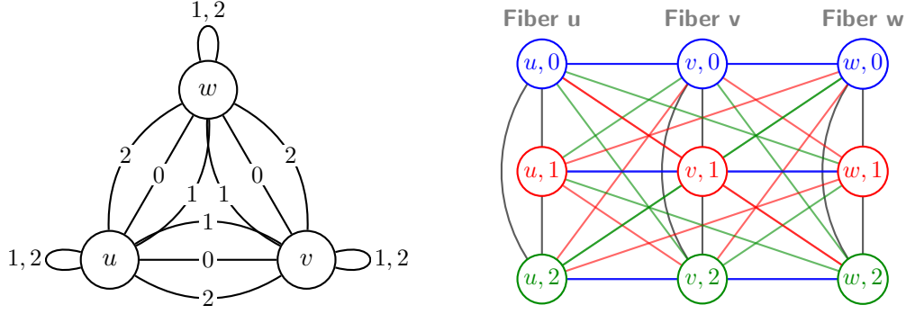
Base \Gamma : full undirected multigraph Derived \Gamma^\lambda : perfect K_{3,3} between all fibers
