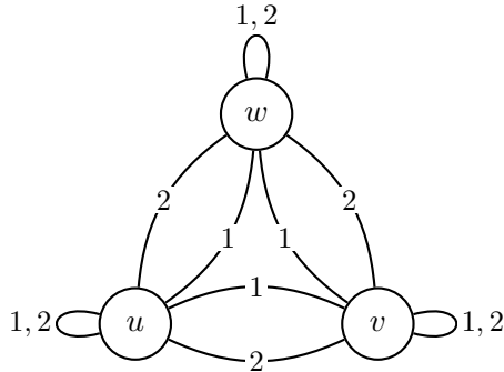
Base \Gamma : undirected multigraph
