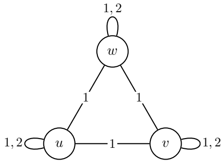
Base \Gamma : undirected triangle & loops
