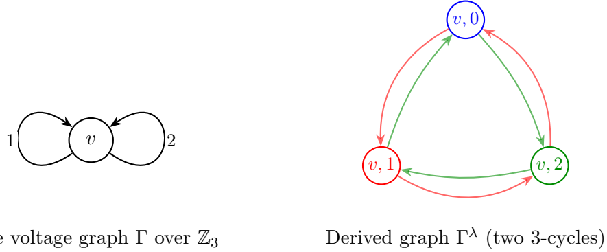
Figure 3.1: Voltage graph and derived cover over \mathbb{Z}_3 , for a base graph with a single vertex and two loops.
