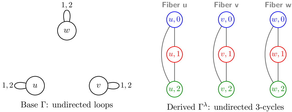
Figure 4.2: Voltage graph and derived cover for the loopfree, undirected quantum graph on M_3 with m = 2 quantum edges.
