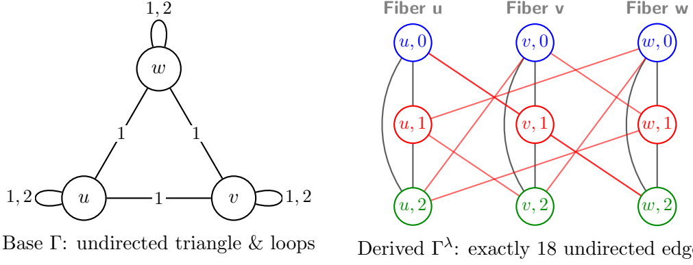
Figure 4.3: Voltage graph and derived cover for the loopfree, undirected quantum graph on M_3 with m = 4 quantum edges.
