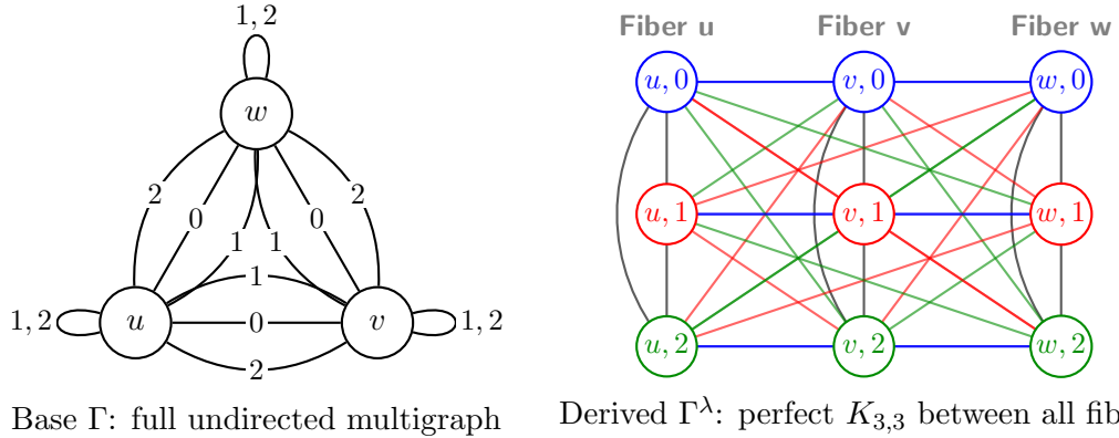
Figure 4.5: Voltage graph and derived cover for the loopfree, undirected quantum graph on M_3 with m = 8 quantum edges.
