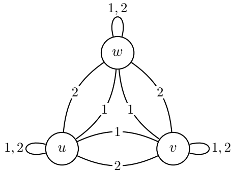
Base \Gamma : undirected multigraph
