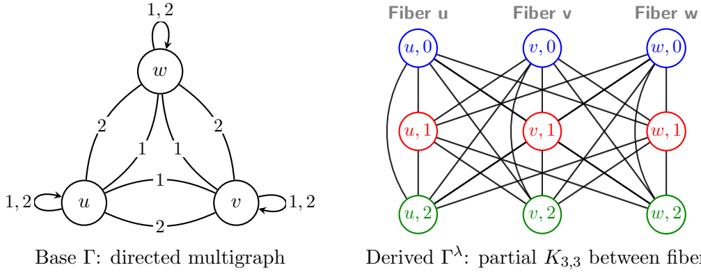
Figure 4.5: Voltage graph and derived cover for the loopfree, undirected quantum graph on M_3(\mathbb{C}) with m = 6 quantum edges.
