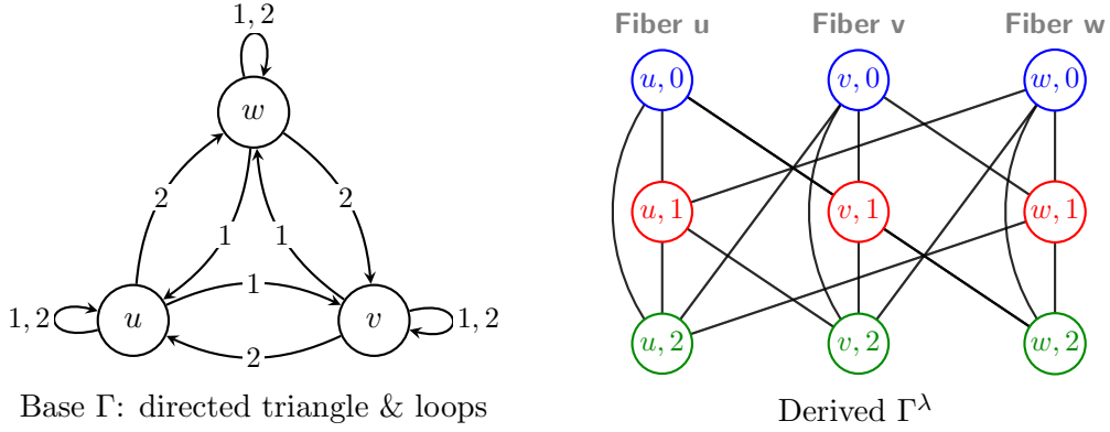
Figure 4.4: Voltage graph and derived cover for the loopfree, undirected quantum graph on M_3(\mathbb{C}) with m = 4 quantum edges.
