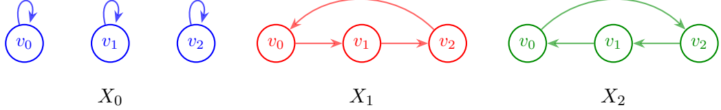
Figure 3.5: The graphs corresponding to the adjacency matrices X_g .
