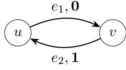
Figure 3.1: Base voltage graph \Gamma over \mathbb{Z}_2
