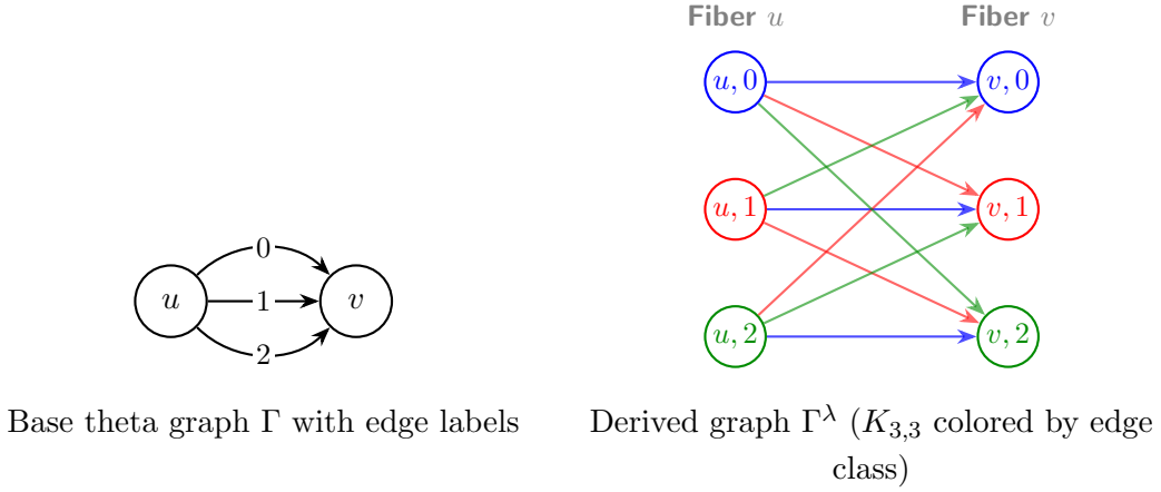
Figure 3.3: Voltage graph and derived cover for a theta graph over \mathbb{Z}_3 .
