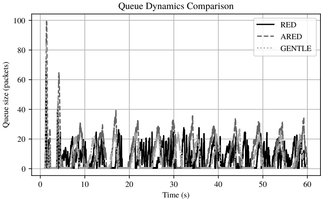
Figure 4. Queue length dynamics for RED, ARED, and Gentle RED
