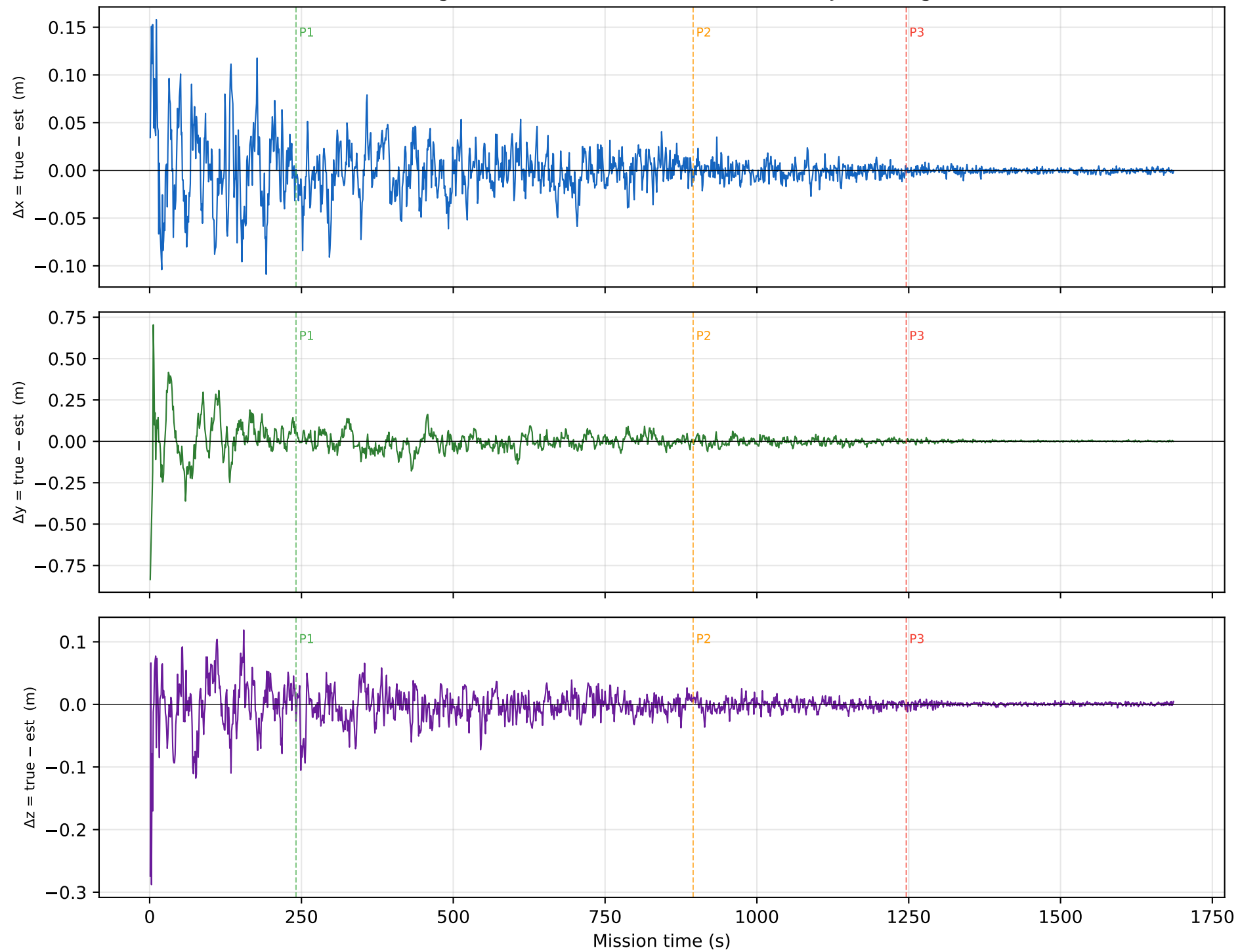
Navigation Error (True - Estimated) under J2 + Drag
