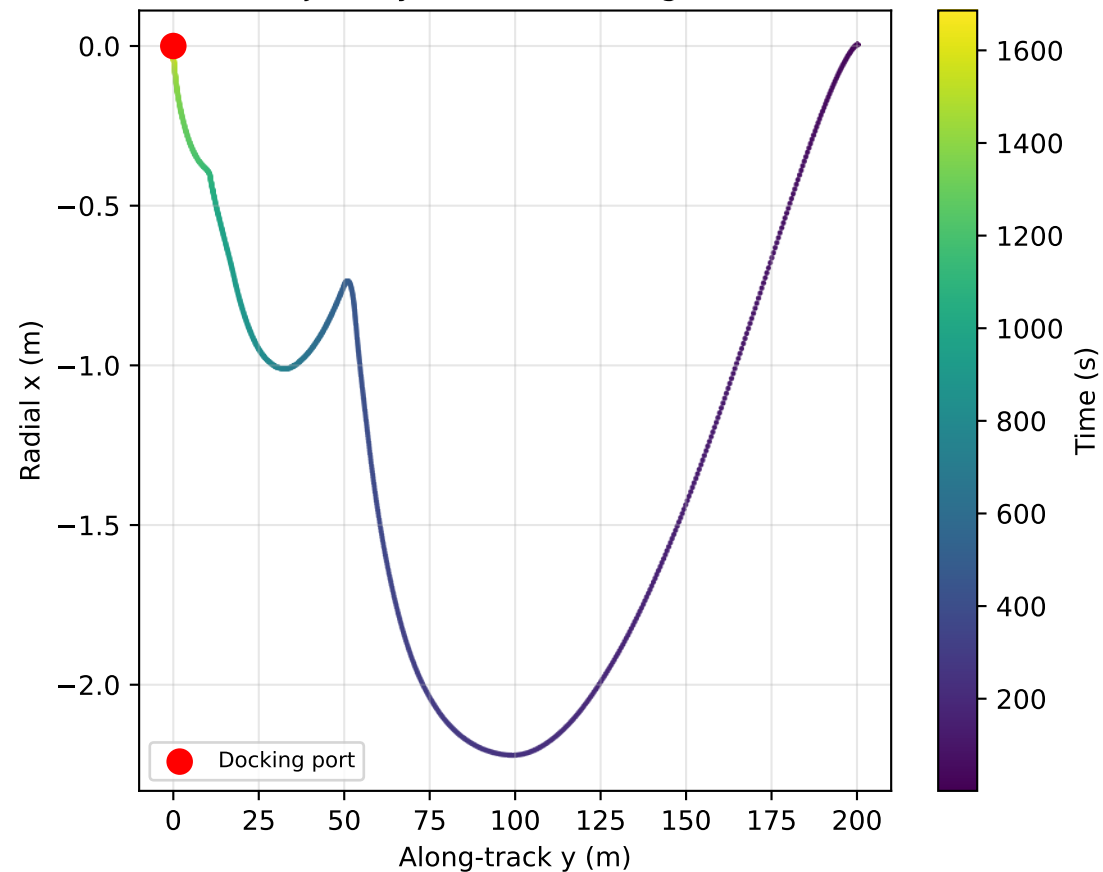
Trajectory: Radial vs Along-track
