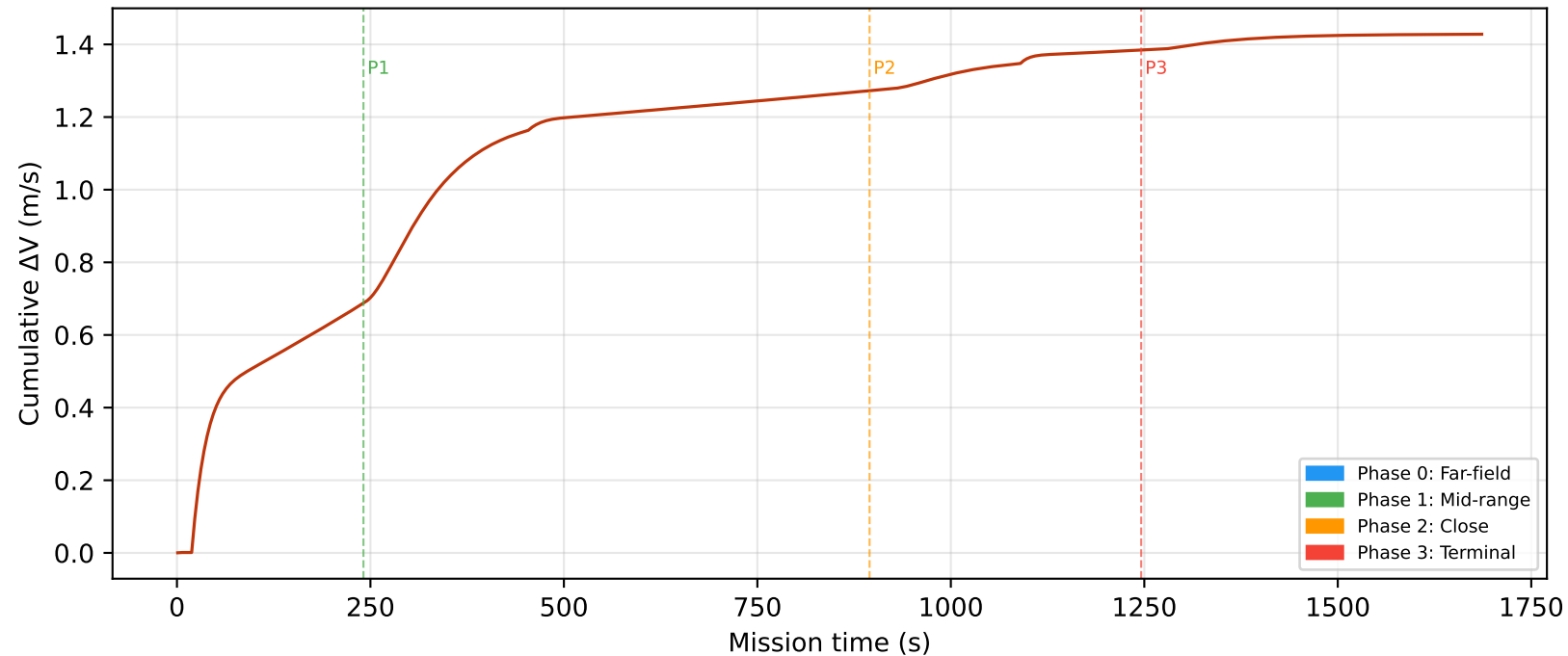
\Delta V Budget vs Time
