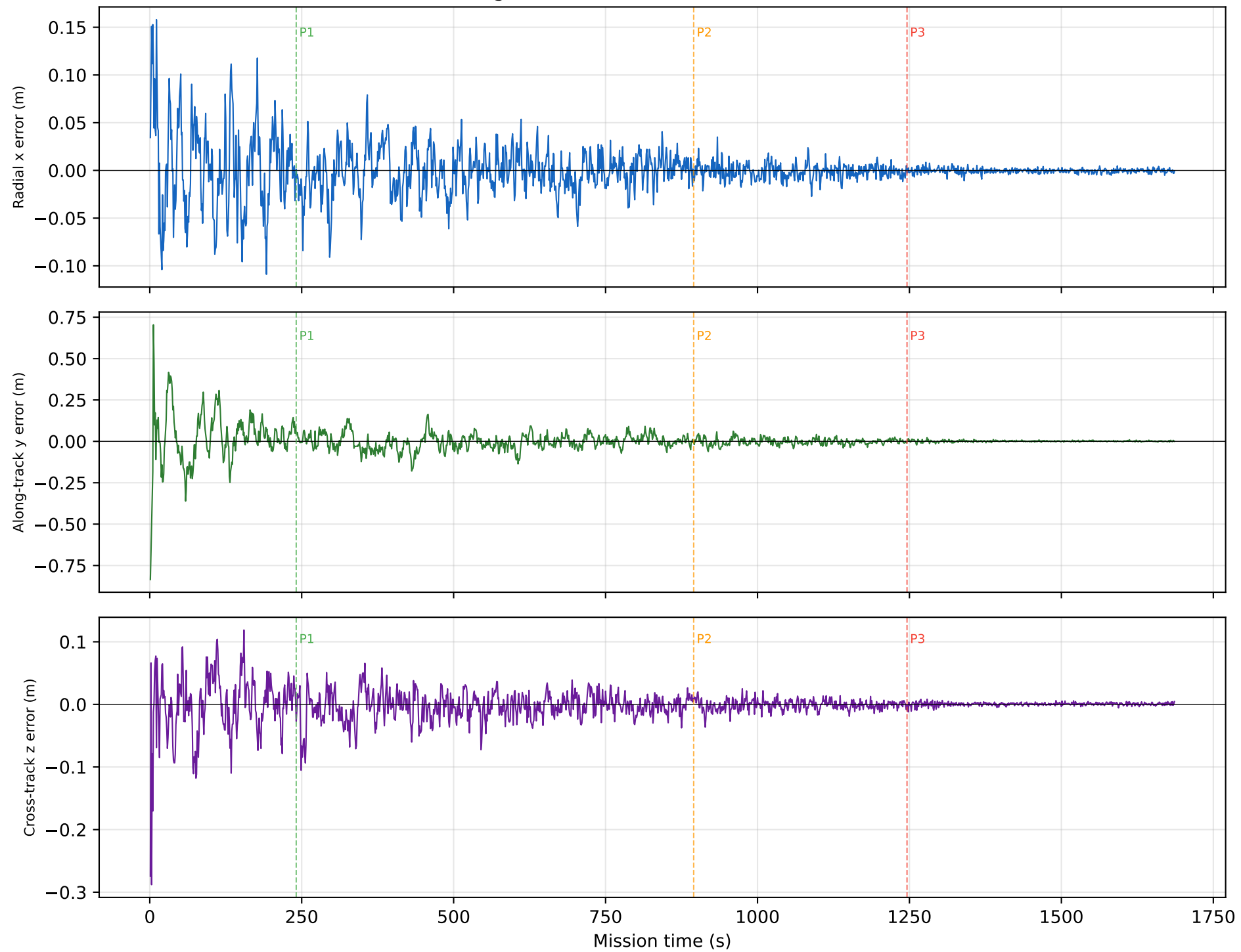
Navigation Filter Error (true – estimated)
