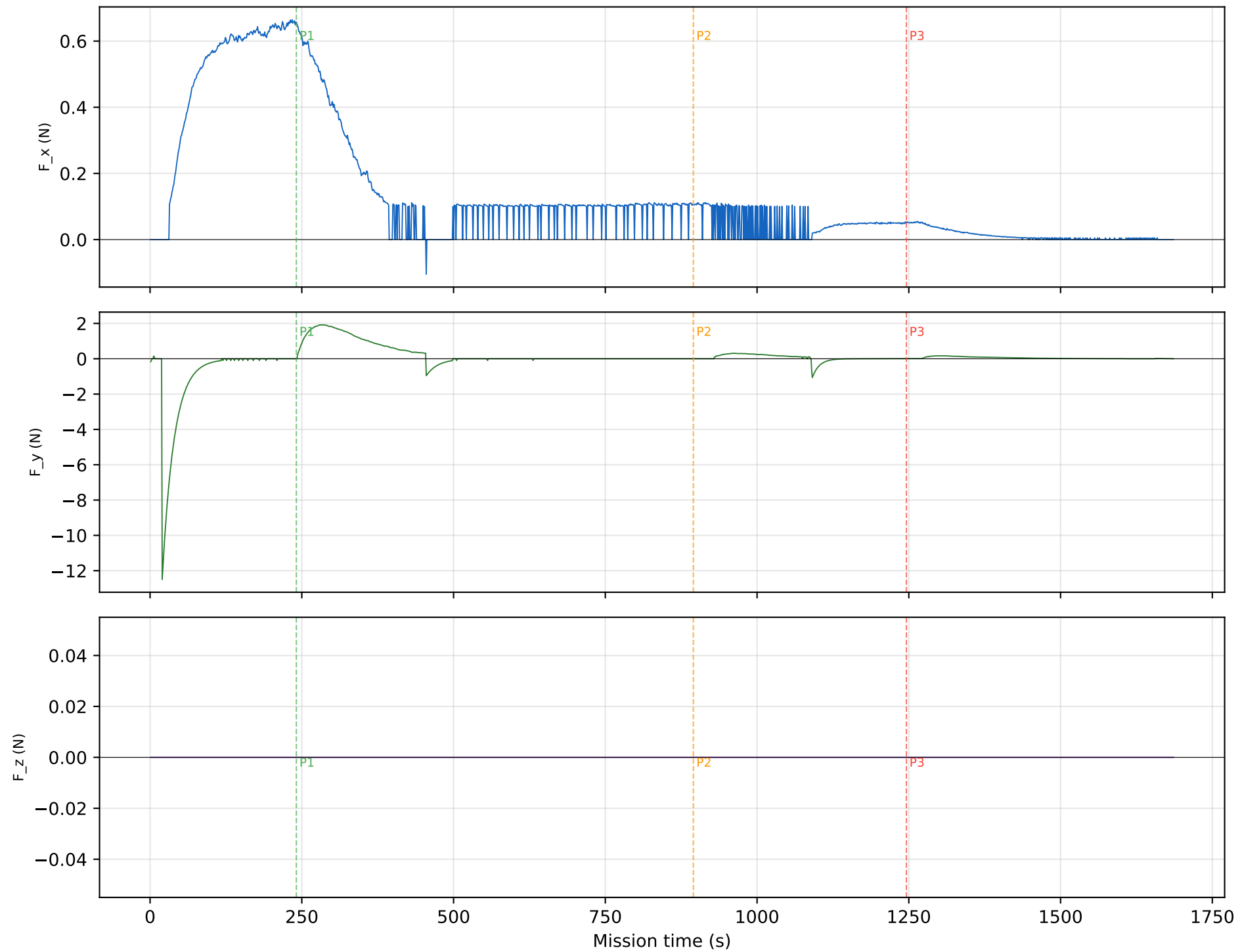
Thruster Command vs Time
