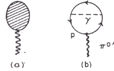
FIG. 1. (a) The general scalar meson tadpole diagram. (b) A typical \pi'^0 tadpole, due to electromagnetism.
