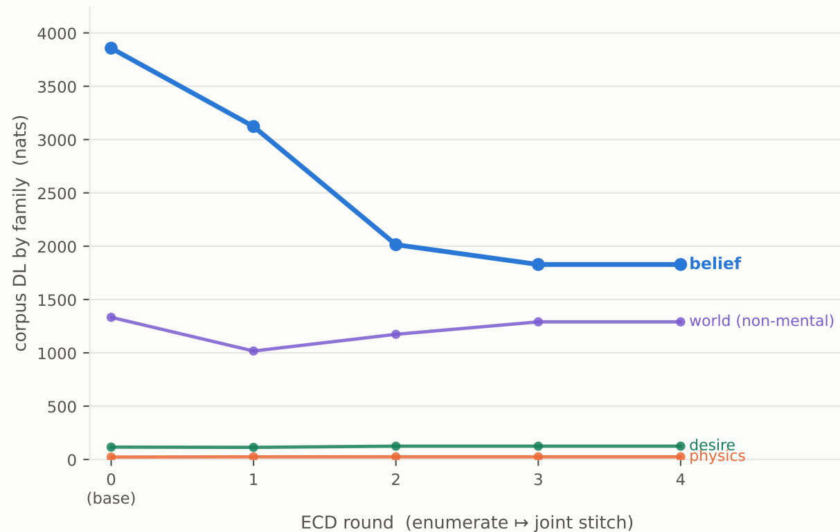
per-family contribution
