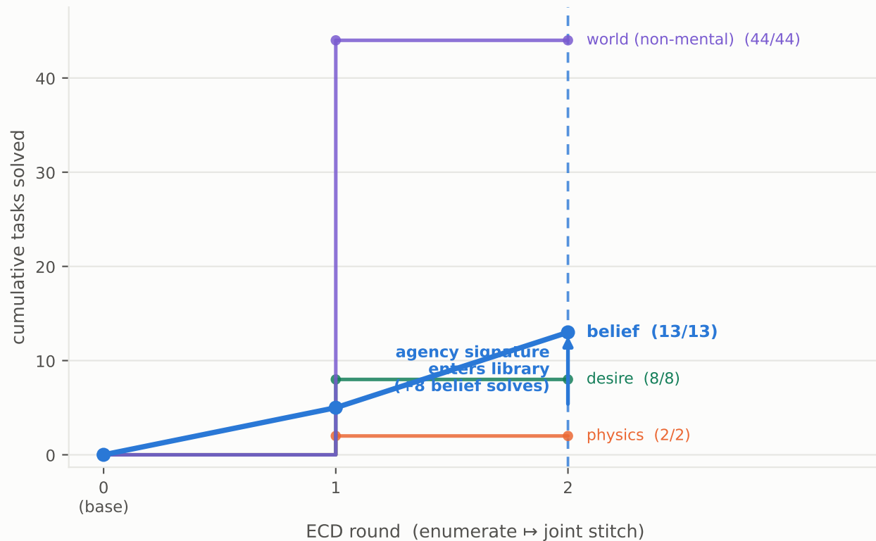
Phase 1 — atomic fork/sync (cumulative solves)
