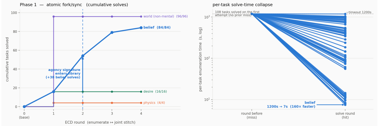
Figure 5: Cumulative solves by task family (atomic primitives)
