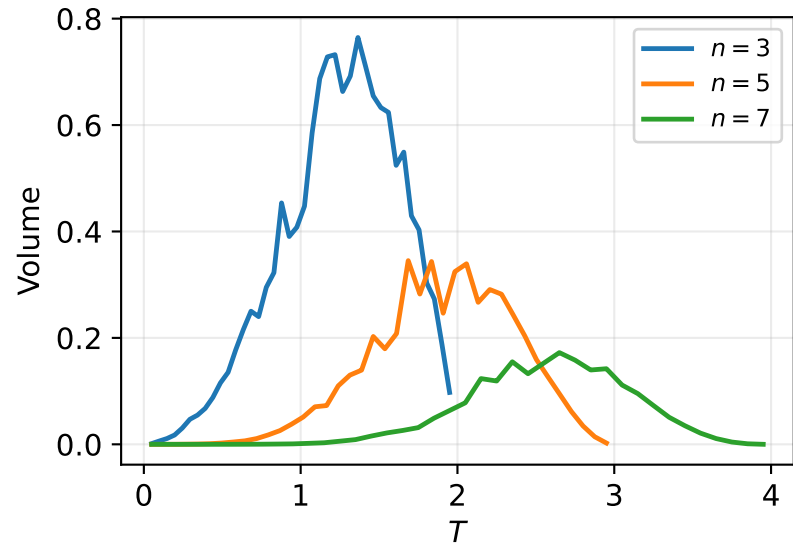
True union volume V^{e_{\text{ex } \cup}} = V^{\mathcal{M}} - V^{e_{\text{ex } n}}
