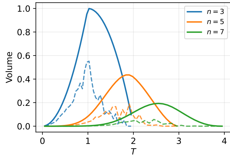
V^{\mathcal{M}} (solid) and V^{e_{\text{ex } n}} (dashed)
