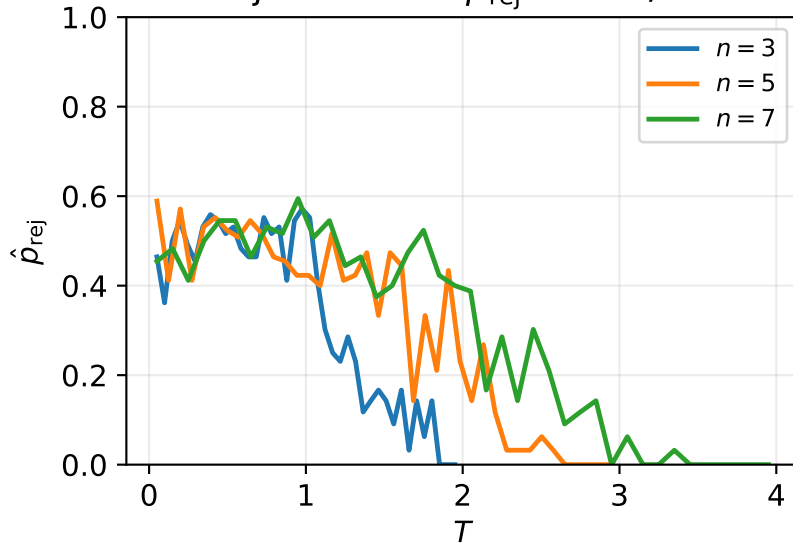
Rejection rate \hat{p}_{\text{rej}} = V^{e_{\text{ex } n}} / V^{\mathcal{M}}
