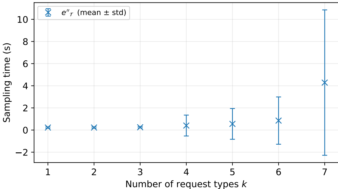
e''_{\mathcal{T}} : sampling time vs k ( n = 10 , T free)
