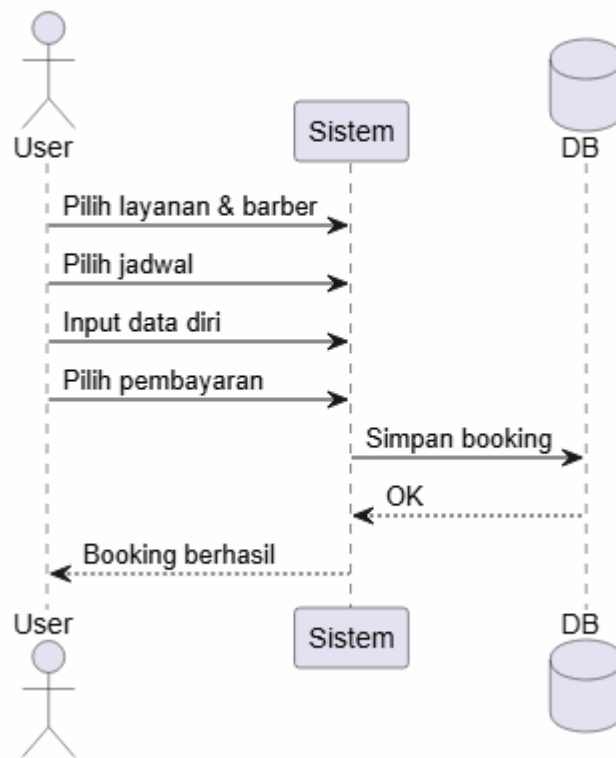
Sequence Diagram - User Booking
