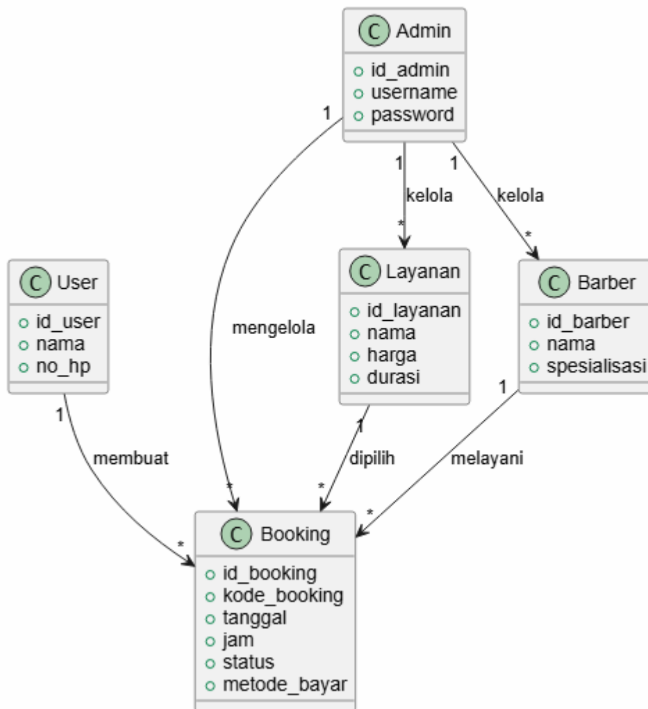
Class Diagram Barbershop (User & Admin)
