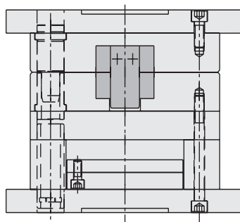
Mounting Example
