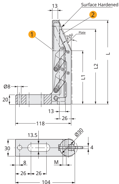
Guide for Sensor - Hardened
