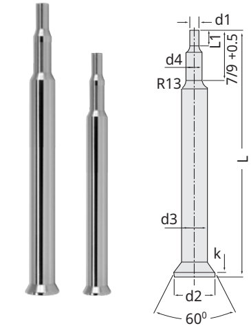
DIN 9861 Form E Conical Head Punches Stepped Code: H2K
