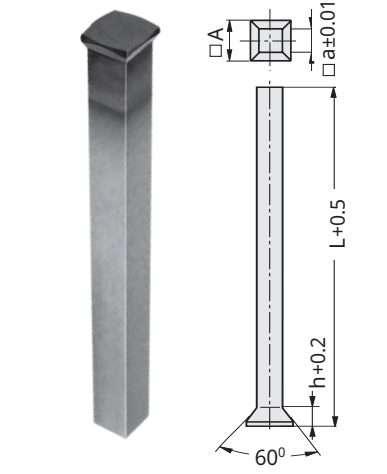
Slot - Form DA forged head Square Head Punch, Slot Stepped Code: HFK
