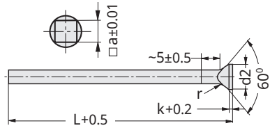
Conical Head Punch Shaped Code: HFY
