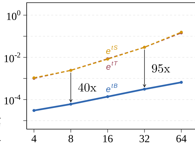
Matrix exponential
