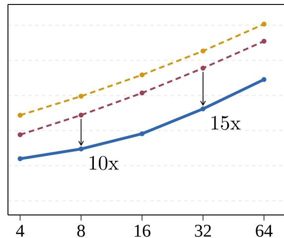
Lyapunov equation
