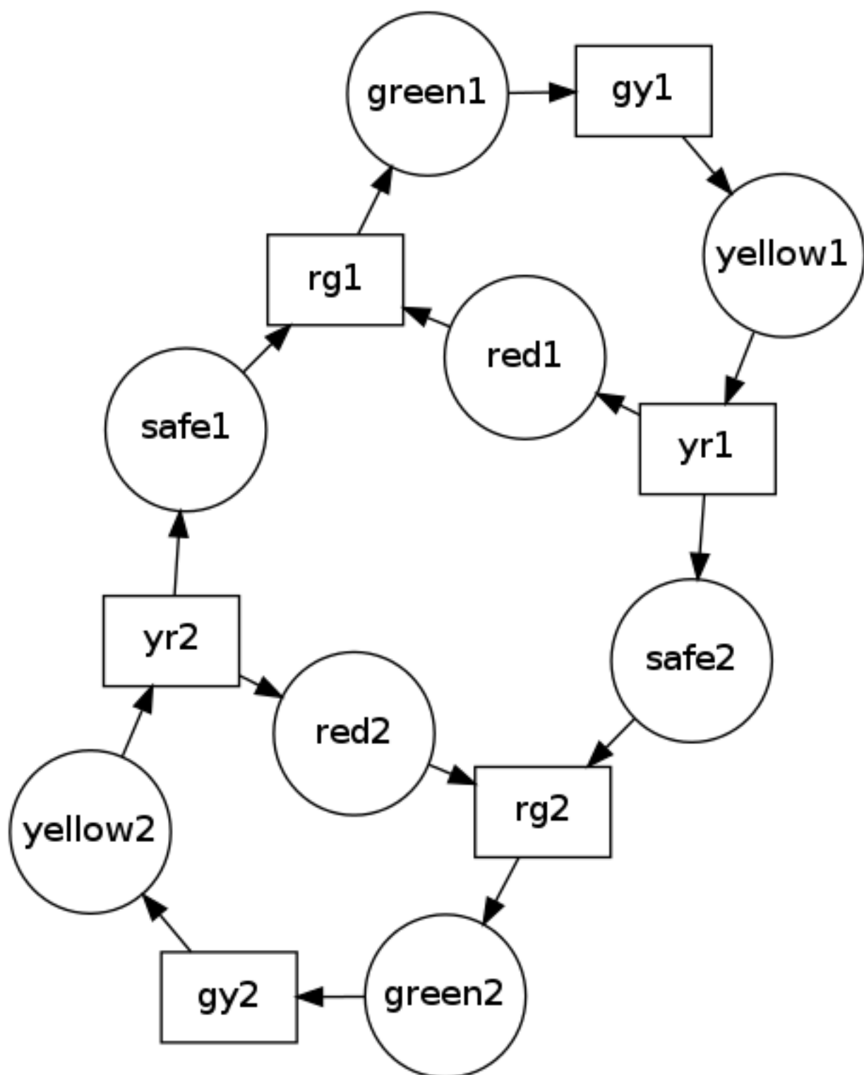
PetriNet Model TrafficLights
