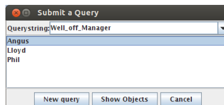
Figure 8.9: Query dialog
