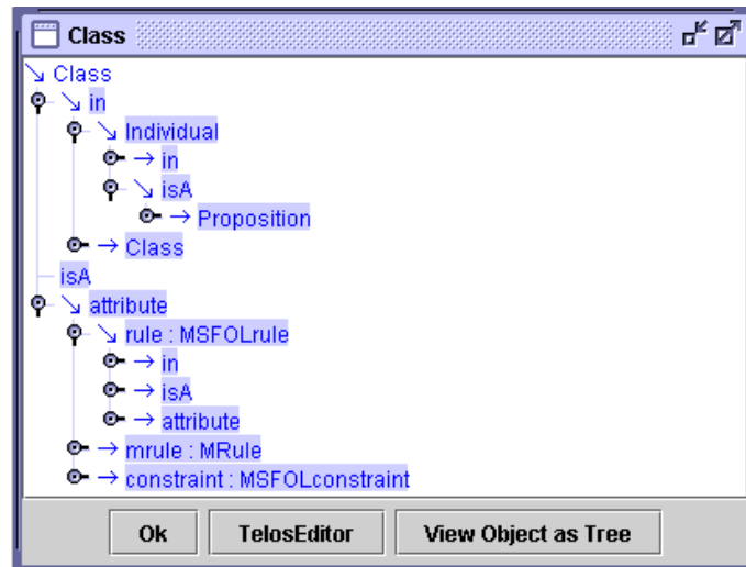
Figure 8.6: Tree Browser
