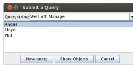
Figure 8.9: Query dialog
