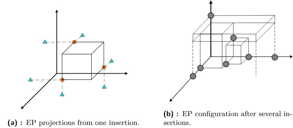
Figure 3.1: Illustration of Extreme Point generation and accumulation[ARCO22]
