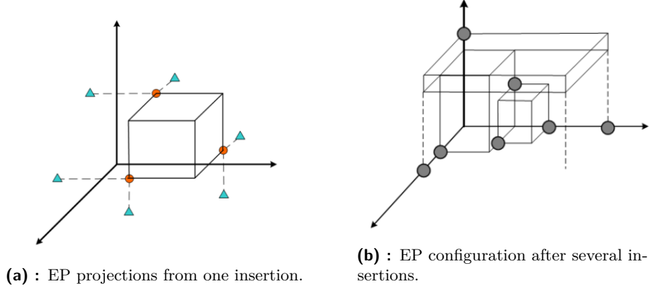
Figure 3.1: Illustration of Extreme Point generation and accumulation directly from the paper
