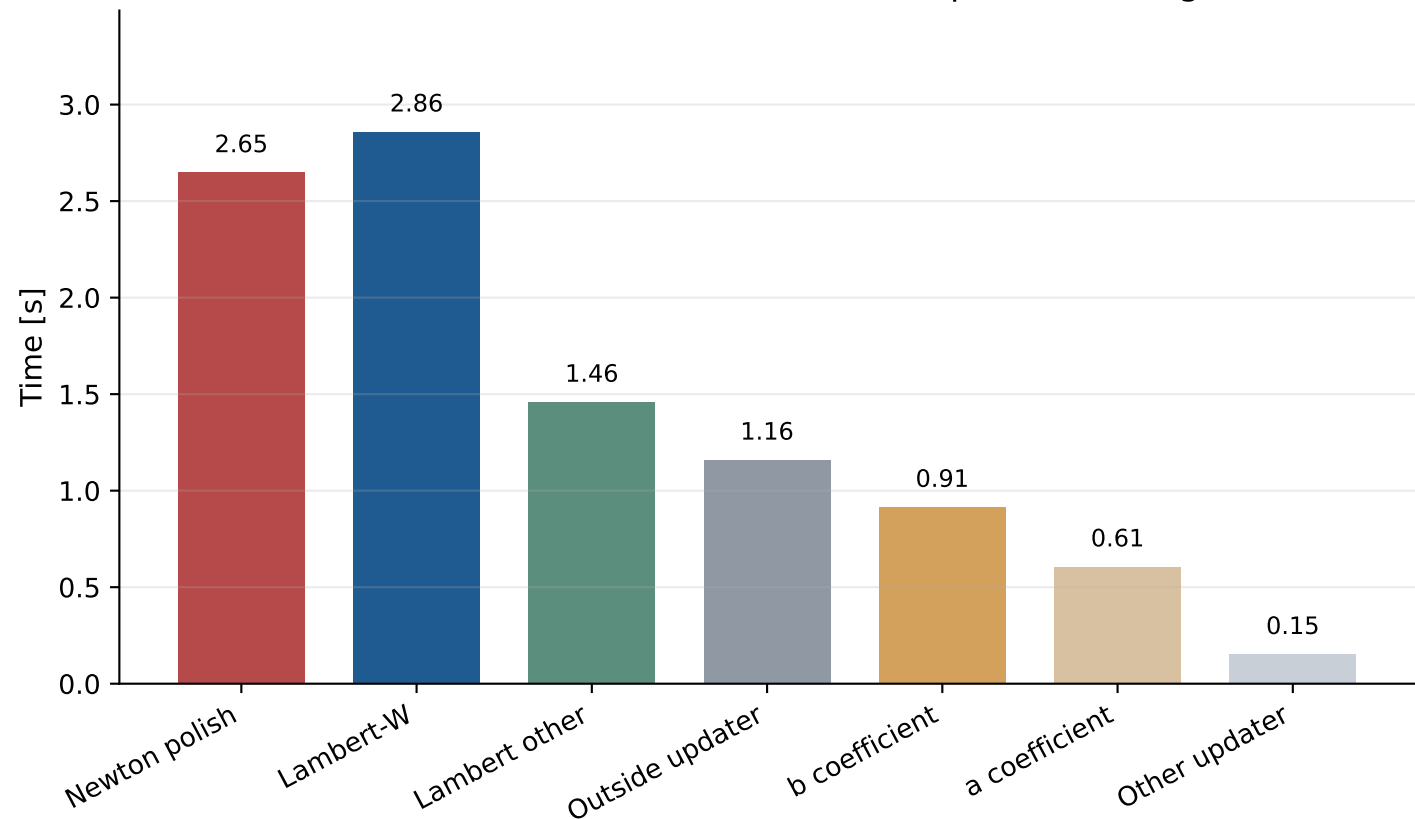
Double-Diode 3H/128: Float64 Component Timing
