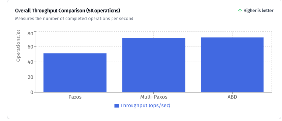
Figure 1: Overall Throughput Comparison (5K operations)
