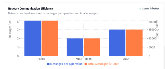
Figure 3: Network Communication Efficiency
