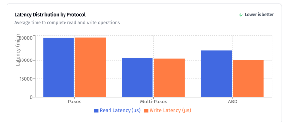
Figure 2: Latency Distribution by Protocol
