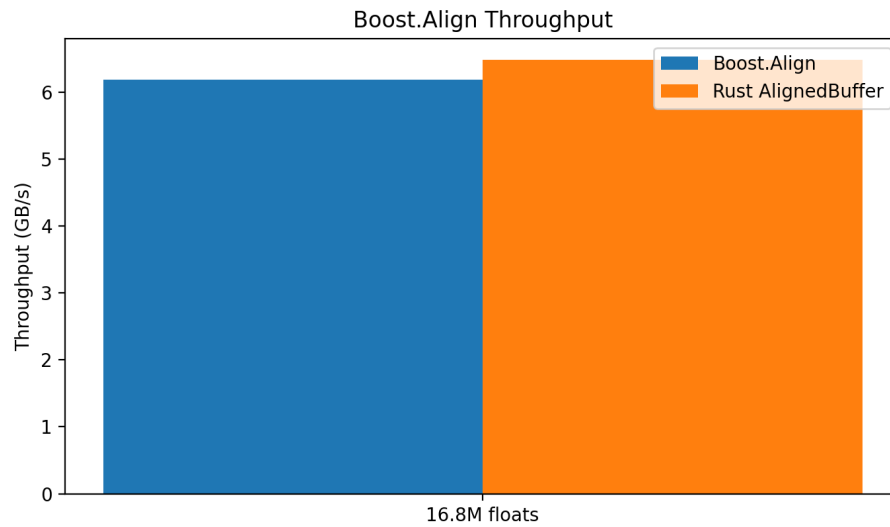
FIGURE 6.2: Measured Boost.Align throughput
