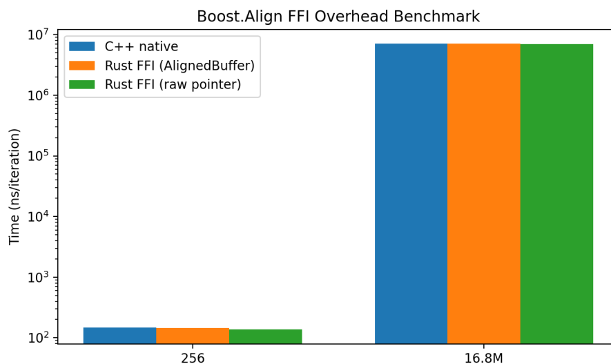
FIGURE 6.3: Selected Boost.Align FFI-overhead measurements; logarithmic vertical scale
