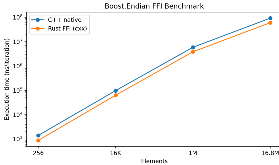
FIGURE 6.4: Boost.Endian measured execution time across input sizes
