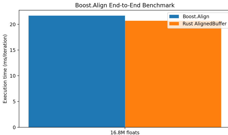
FIGURE 6.1: Measured Boost.Align end-to-end execution time
