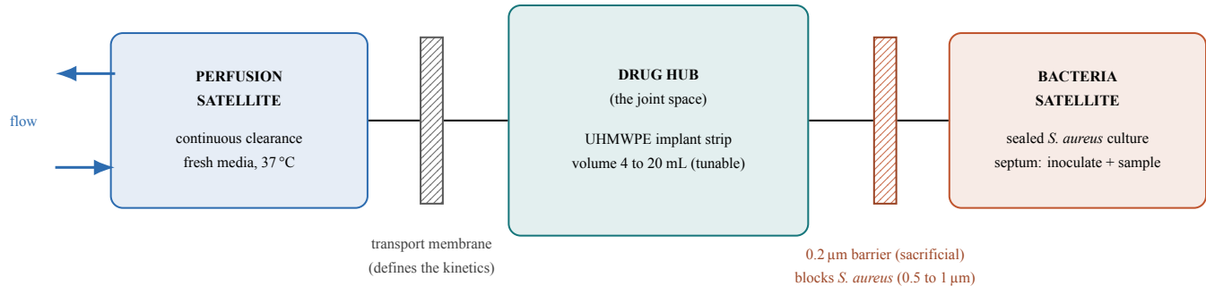
Figure 1. Radial three-chamber architecture of the DRD-3. The two membranes sit on opposite faces of the central drug hub rather than stacked in series, so biofilm that is allowed to form on the sacrificial 0.2 µm barrier on the infection side cannot reach the transport membrane that defines the release kinetics. The full device seals on three identical O-ring pairs (2.0 mm cord, 1.5 mm gland, 25% compression) across three interface types (cartridge-to-satellite, lid-to-base, satellite-to-hub); each satellite is drawn to the hub by a two-piece C-ring wrapper with one bolt per side.
